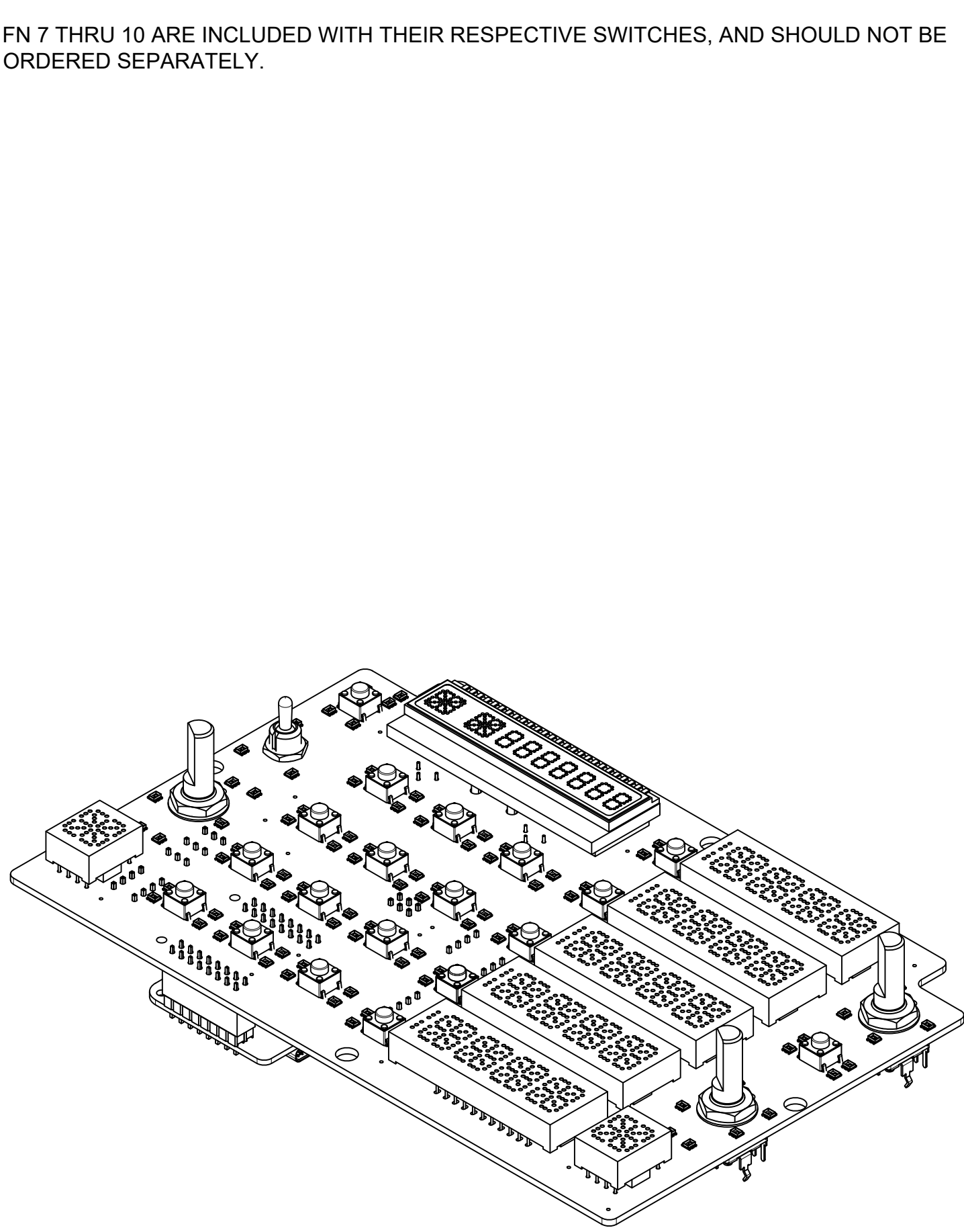
-1 ASSY SCALE 1:1
