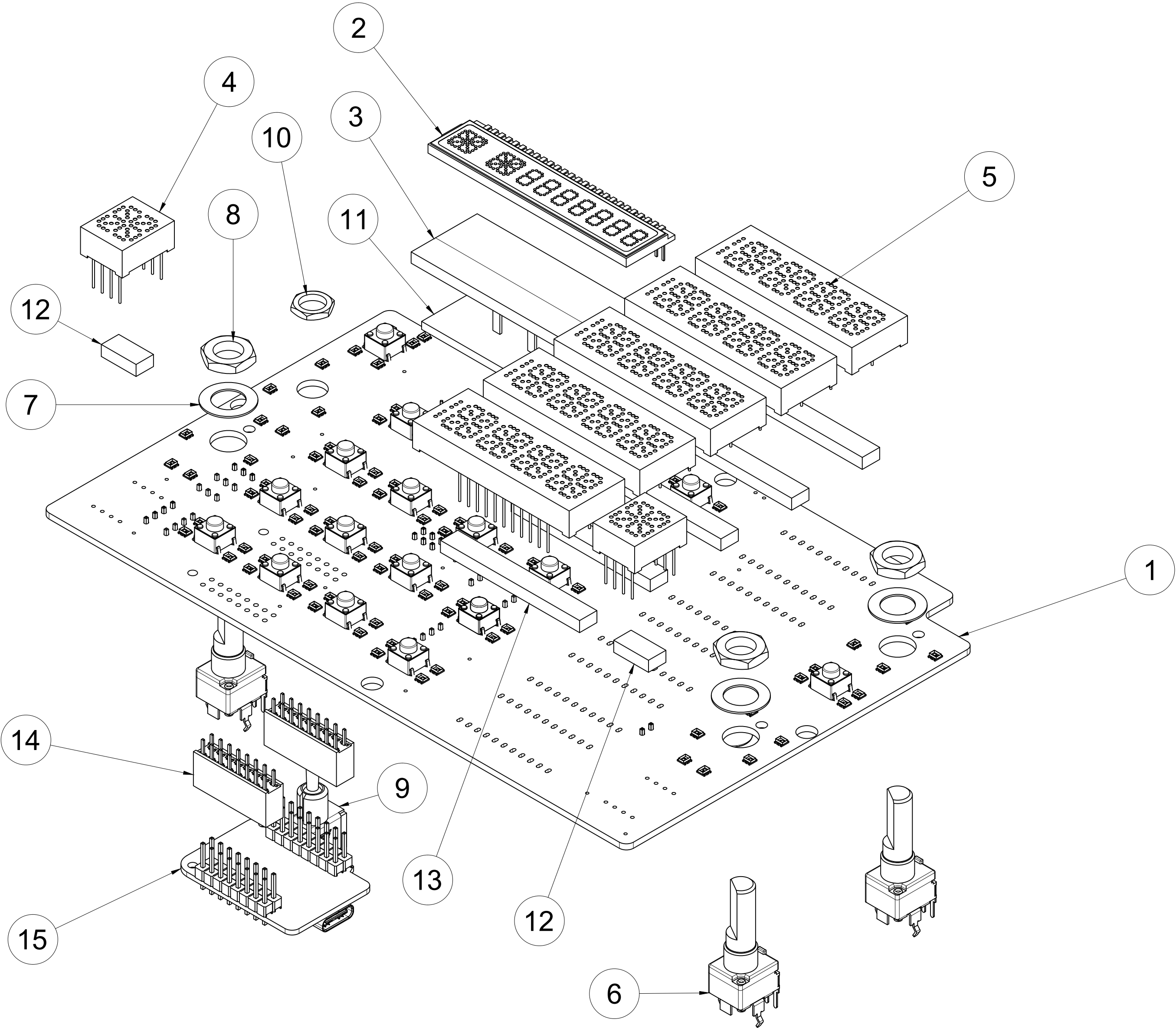
-1 ASSY
